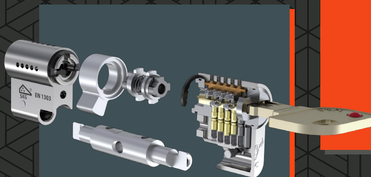
Modular system
